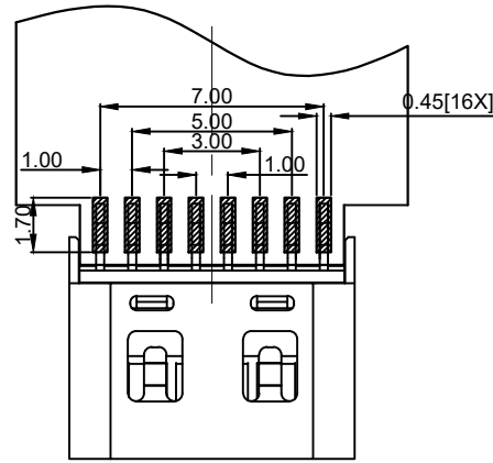
RECOMMENDED P.C.B. LAYOUT T=1.0 ±0.05mm
